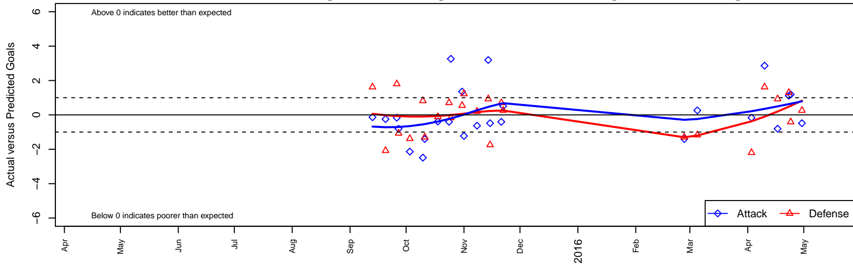
THUSC Copper G04 Dots are actual minus expected GF (blue circles) and GA (red triangles). Blue line is smoothed change in attack strength. Red is smoothed change in defense strength.
